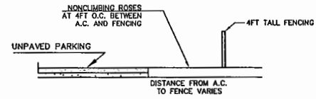
PARKING AREA PERIMETER LANDSCAPE
